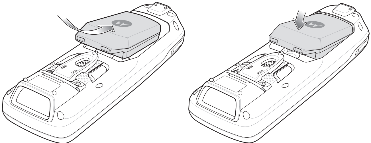
Figure 1-4 Insert Battery
